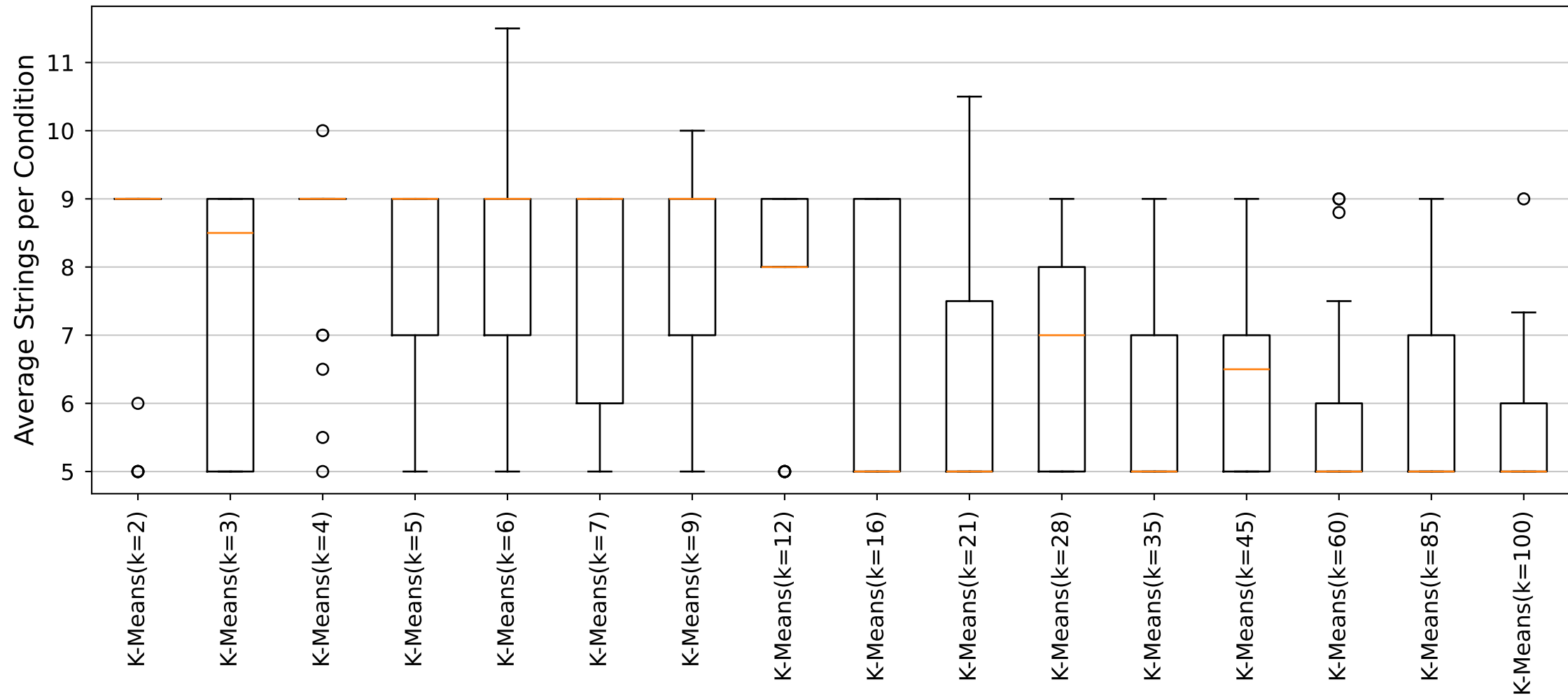
YARA Rules Average Strings per Condition Distribution (Cluster2_Size100 dataset)
